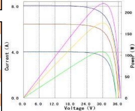
Current, power VS voltage characteristics (solar irradiant: 100%, 80%, 50%)
